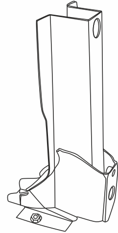
PSMP- 10 Front Flooring Cross No. 1
