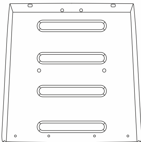
PSMP- 17 Front Tyre Mudguard Big
