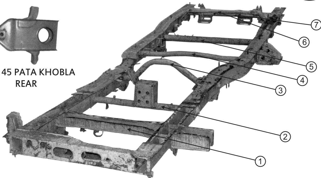
PEW. 44 CHASSES FULL ASSY
